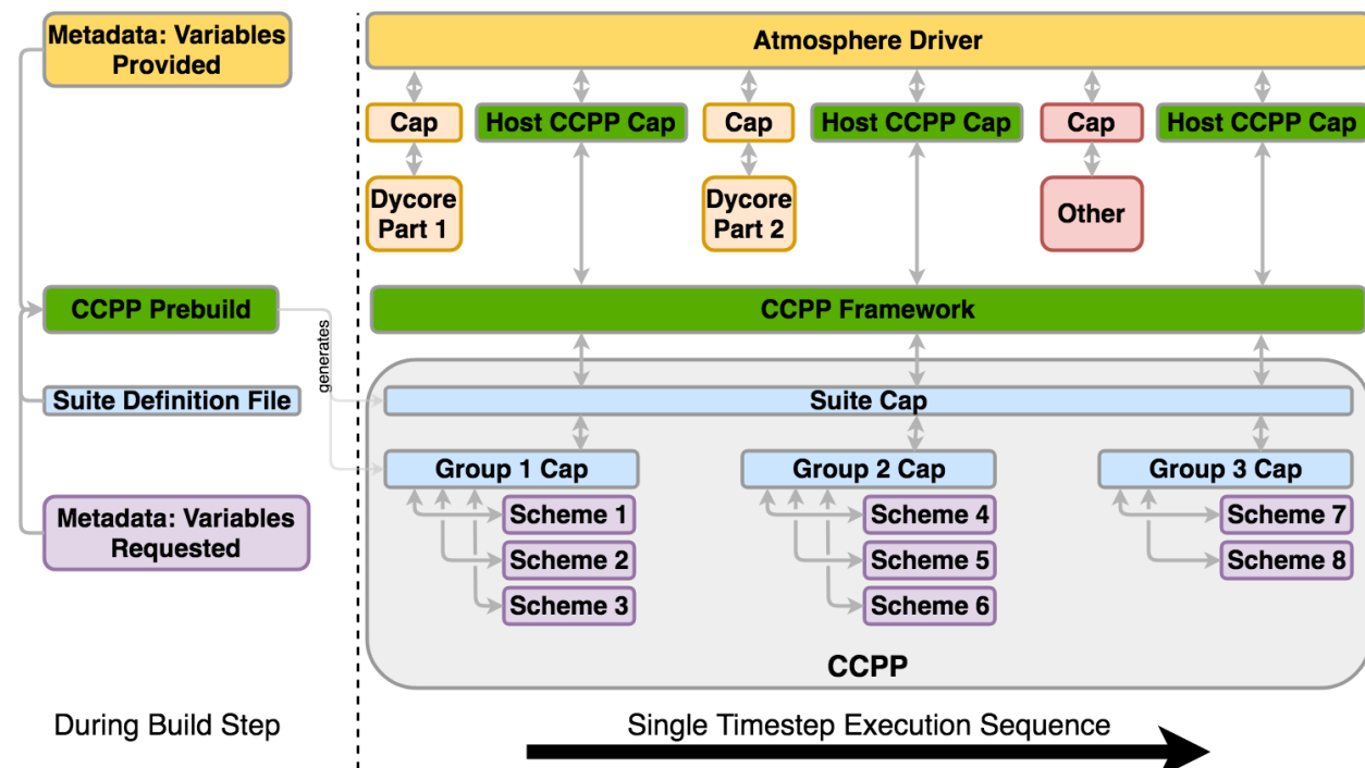
Fig. 3.3: As in Figure 3.2 , but for the static build using a single SDF. In this case, software caps are autogenerated for the suite and physics groups (defined in the SDF provided to the ccpp_prebuild.py script) rather than for individual schemes. The suite must be defined via the SDF at prebuild time. When multiple SDFs are provided during the build step, multiple suite caps and associated group caps are produced, but only one is used at runtime.
