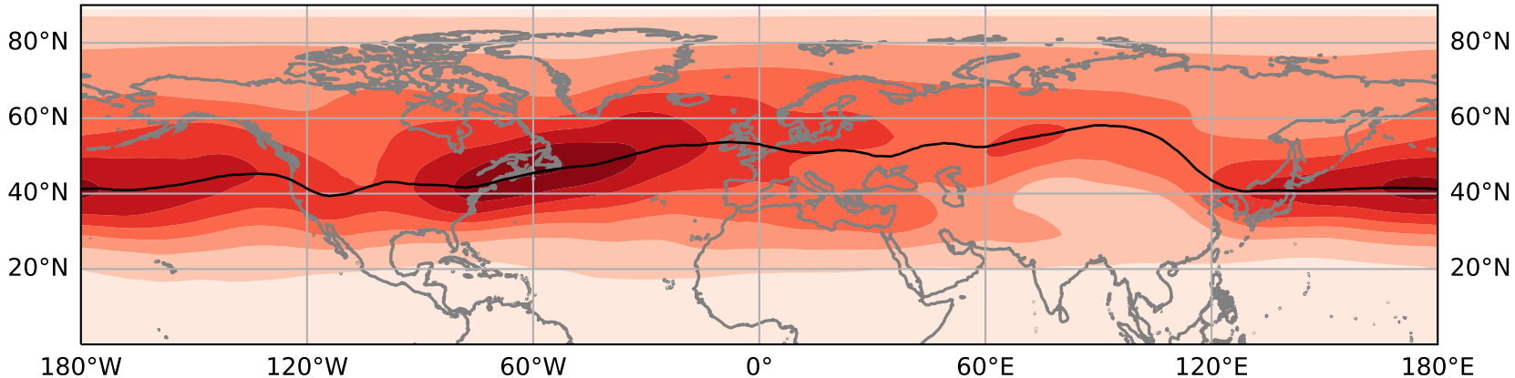
DJF Mean High-Pass Z500 STD
